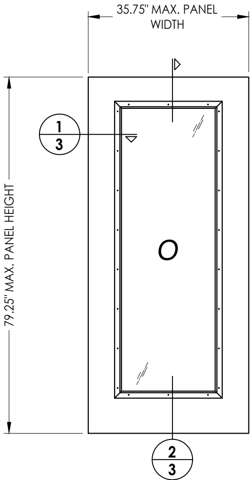
50 FIBERGLASS SIDELITE PANEL BUILDERS HARDWARE
