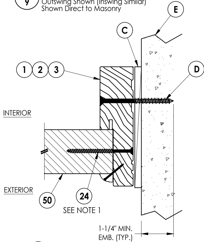
3 HORIZONTAL CROSS SECTION 9 Outswing Shown (Inswing Similar) Shown Direct to Masonry
