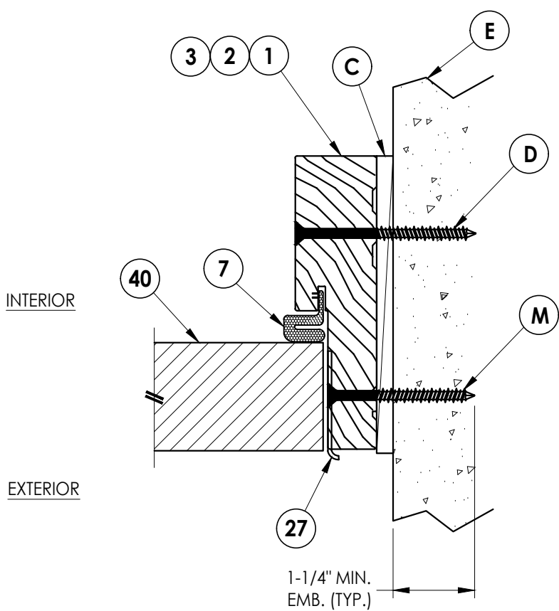
2 HORIZONTAL CROSS SECTION 9 Outswing Shown (Inswing Similar) Shown Direct to Masonry
