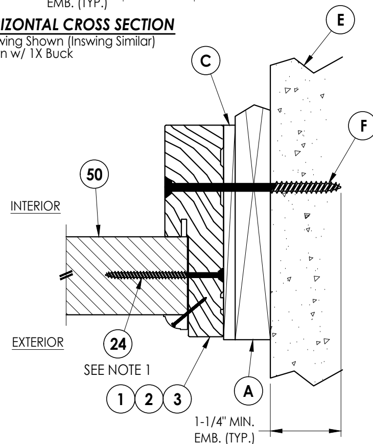
3 HORIZONTAL CROSS SECTION 8 Outswing Shown (Inswing Similar) Shown w/ 1X Buck
