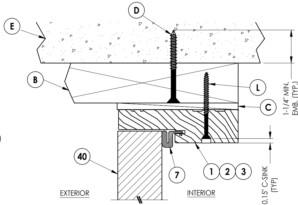
4 7 VERTICAL CROSS SECTION Outswing Shown (Inswing Similar) Shown w/ 2X Buck
