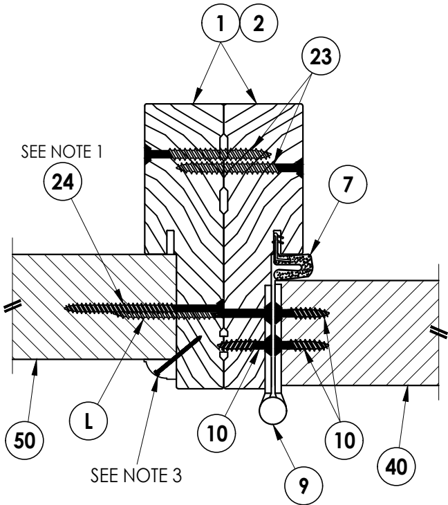
1 6 HORIZONTAL CROSS SECTION Outswing Shown (Inswing Similar)
