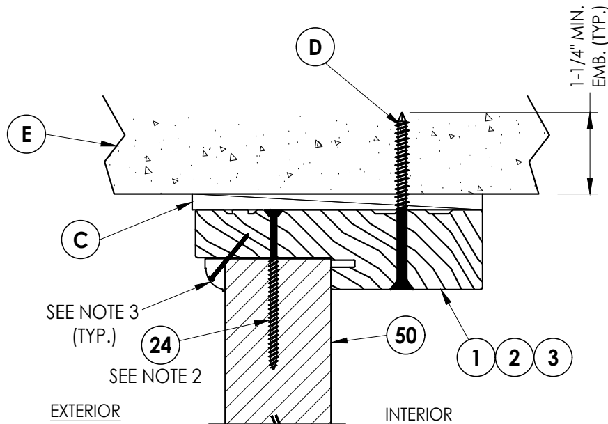
5 VERTICAL CROSS SECTION 9 Outswing Shown (Inswing Similar) Shown Direct to Masonry
