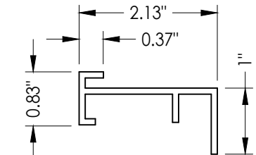
16 INSWING SIDELITE ADAPTER
