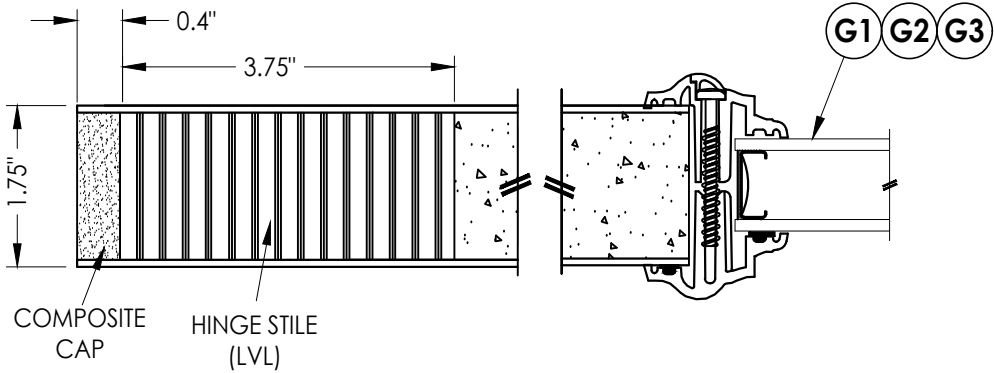
1 HORIZONTAL CROSS SECTION 3
